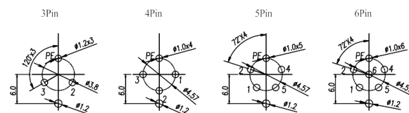
M12 Male Connector C-Coding
