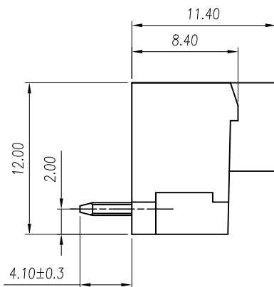
General Tolerances
