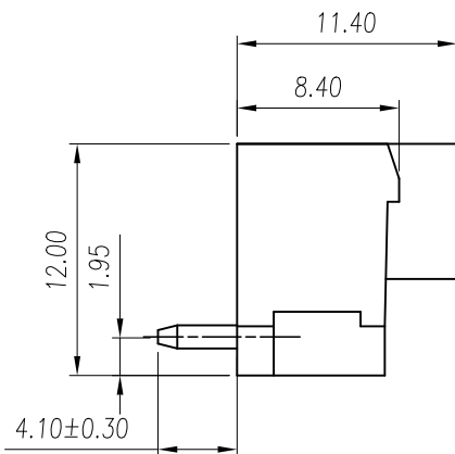
General Tolerances
