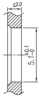
Panel cut-out
