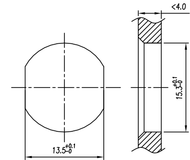
Panel cut-out
