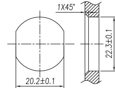
Panel cut-out
