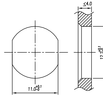
Panel cut-out
