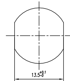
Panel cut-out
