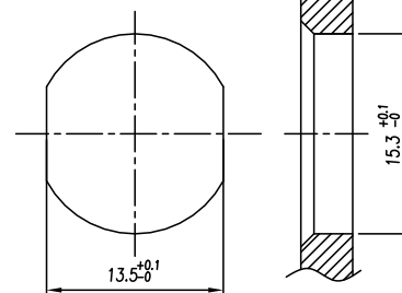
Panel cut-out
