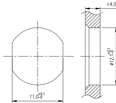
Panel cut-out
