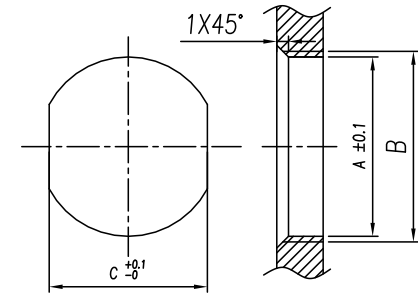
Panel cut-out
