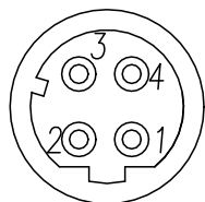
View from front D-CODE 4PIN Female
